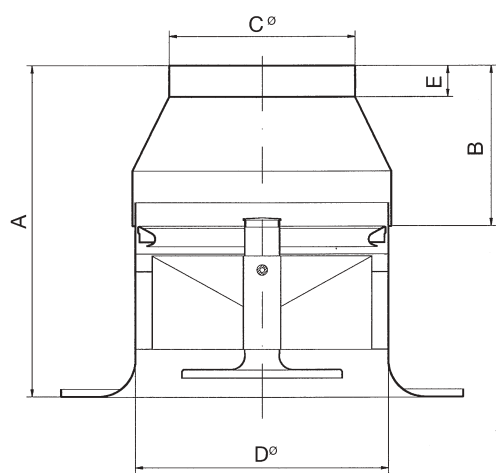
Connection cone
