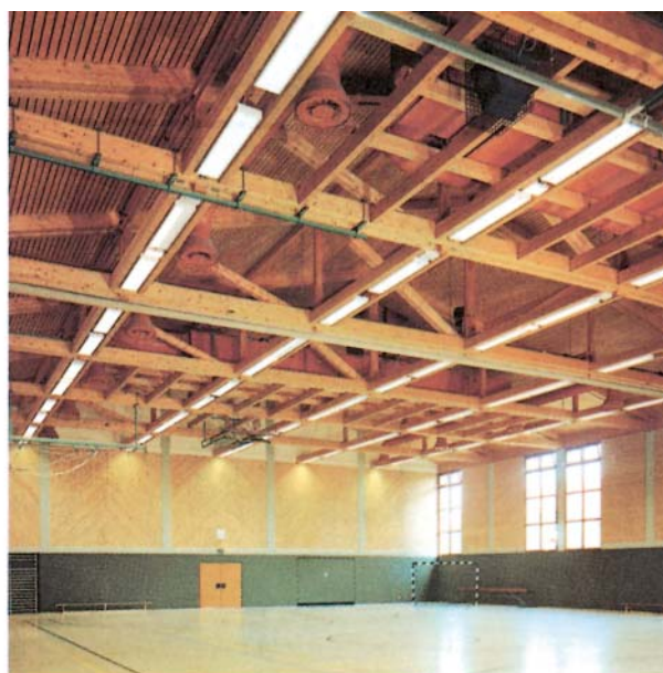
General purpose hall: Kehl-Kork
