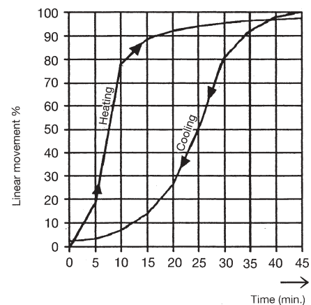
Control response of a self actuating piston
