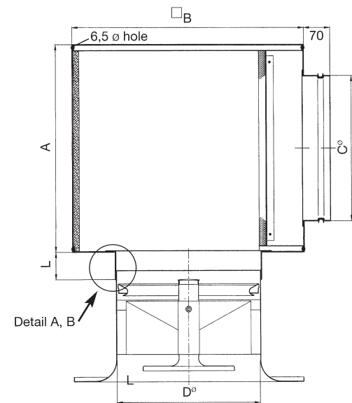
Rectangular connection plenum box
