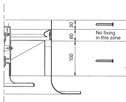
Installation - fixing instruction
