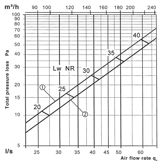
Fig. 5 - WKA 80/30, two way blow
