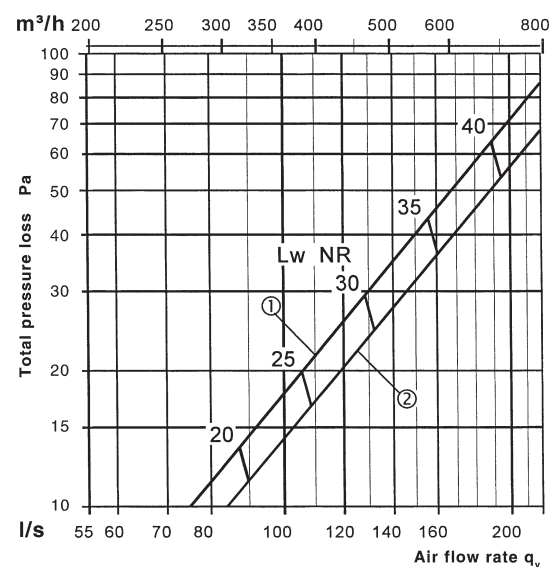
Fig. 7 - WKA 155/45, two way blow
