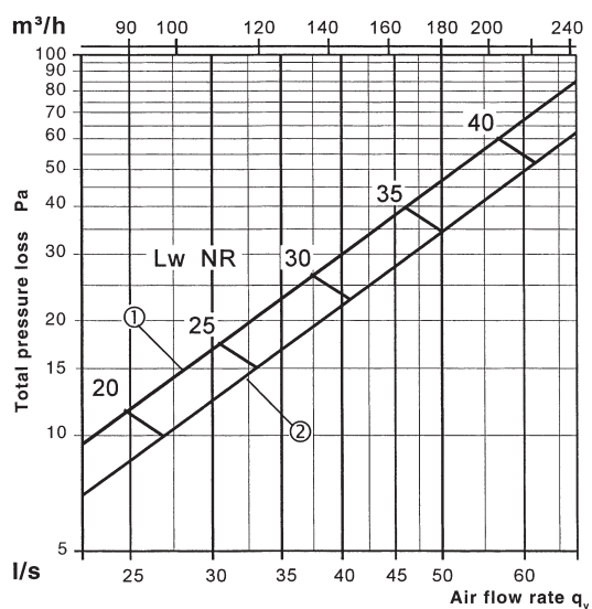
Fig. 4 - WKA 80/30, one way blow
