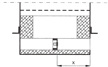
Fig. 8: One way blow linear swirl diffuser WKA-1 with setting element
