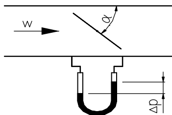
Chart 7.1.1. Pressure losses dependent on the turning of the damper's leaf
