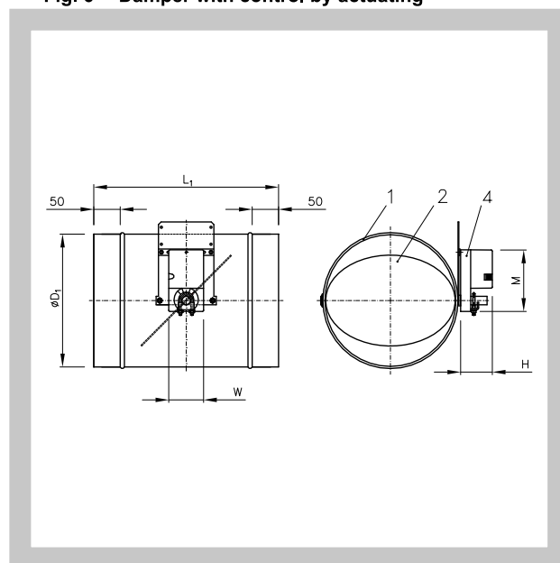
Fig. 6 Damper with control by actuating
