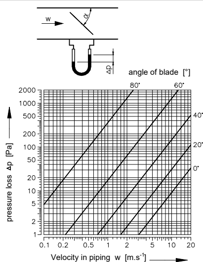
Chart 7.1.1. Pressure losses dependent on the turning of the damper's leaf
