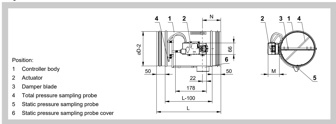
Fig. 5 RPM-LV with insulation
