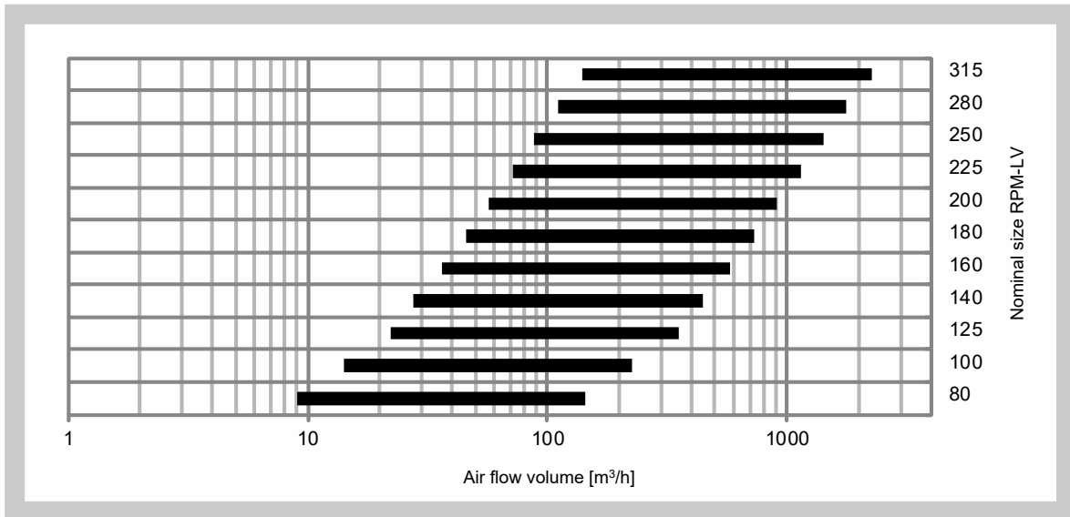
Fig. 16 Controller size selection according to air flow [m 3 /h]
