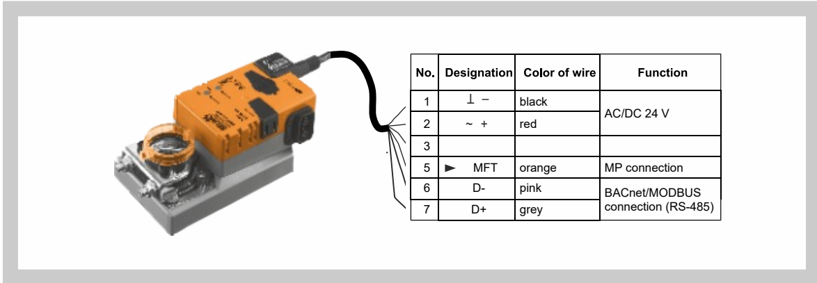
Fig. 9 Actuators LMV-D3-MOD, NMV-D3-MOD and SMV-D3-MOD
