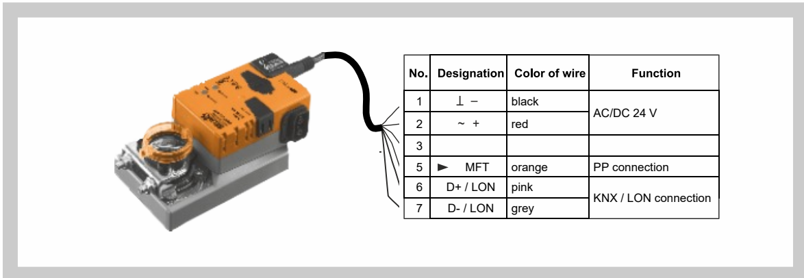
Fig. 12 Wiring of actuators LMV-D3-KNX and NMV-D3-KNX
